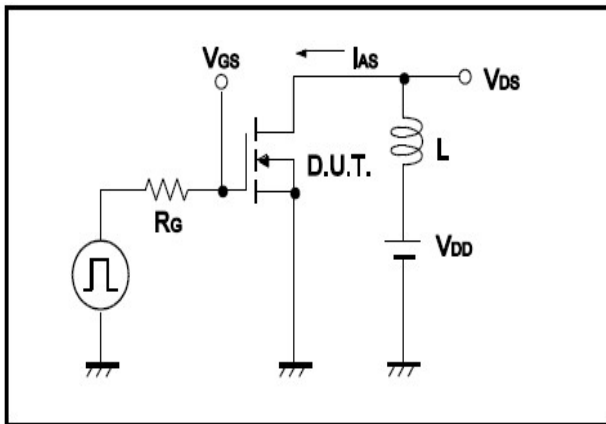
Fig.12 Avalanche Measurement Circuit
