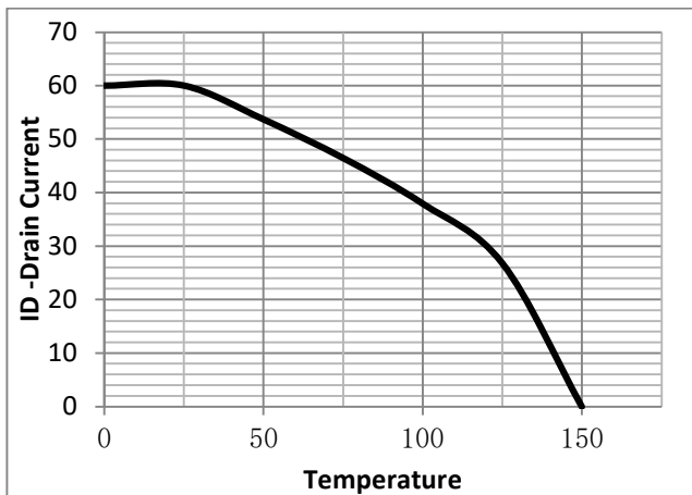
Fig.7 ID V.S Junction Temperature
