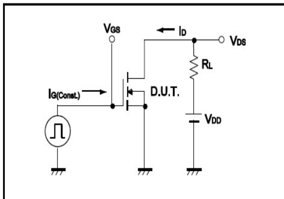
Fig.8 Gate Charge Measurement Circuit
