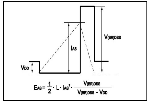
Fig.13 Avalanche Waveform
